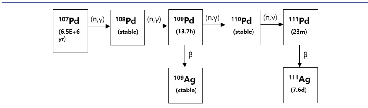
| Pd-107 핵종변환(Pd-108) |
